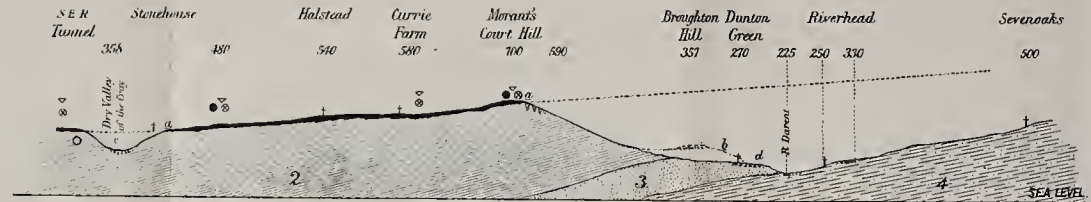
FIG. 1. SECTION FROM THE UPPER PART OF THE CRAY VALLEY TO SEVENOAKS.
